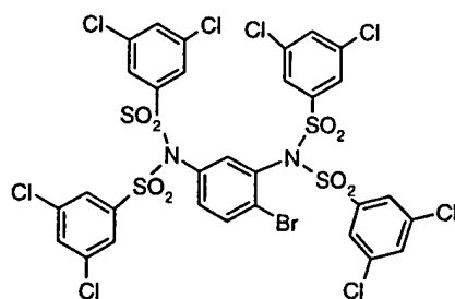
Compound # 30
